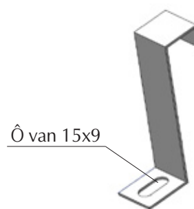
Pass kẹp Z Hold down clamp
