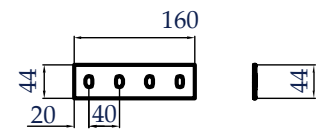
PASS NỐI H = 50mm
