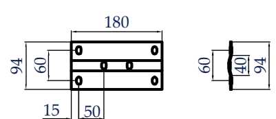
PASS NỐI H = 100mm
