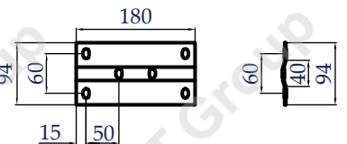
PASS NỐI H = 100mm
